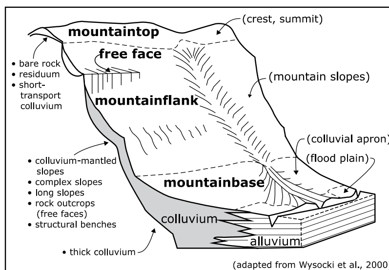
Three-dimensional depiction of geomorphic components of mountains.
