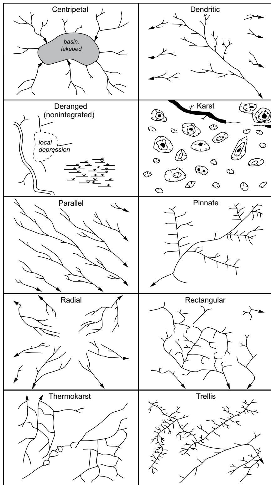
Illustrations and descriptive terms for drainage patterns.
