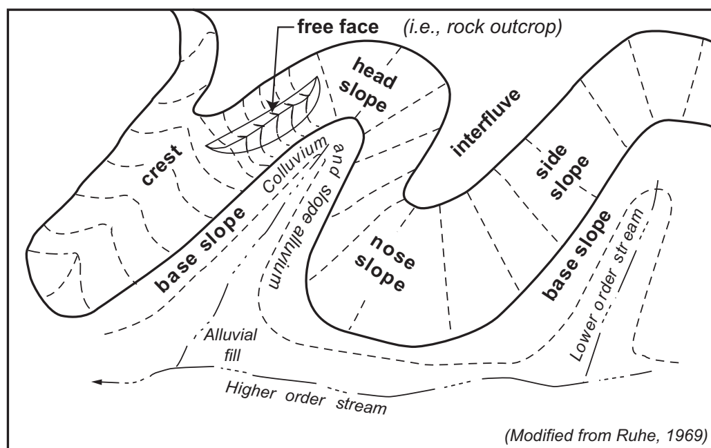
Three-dimensional depiction of geomorphic components of hills.
