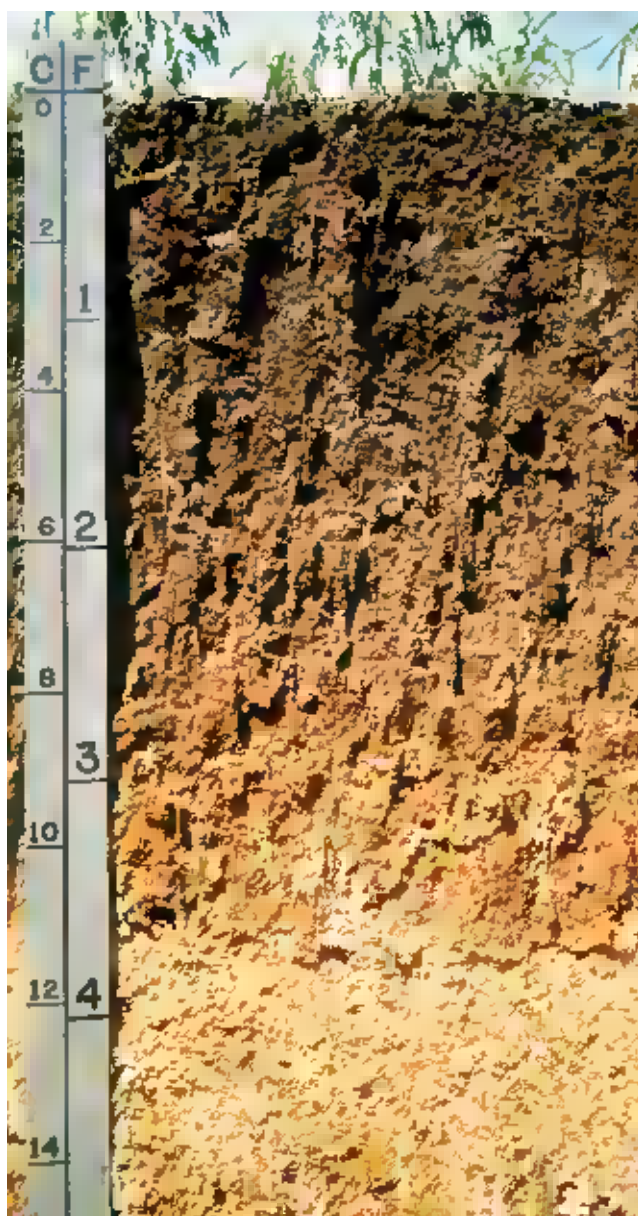
Profile of the Olton series.
